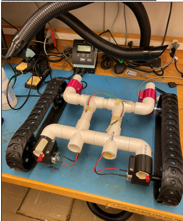
Robot frame with electrical motors installed.
